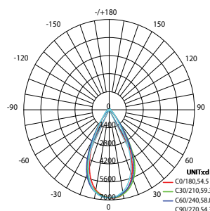
Beam angle 60
